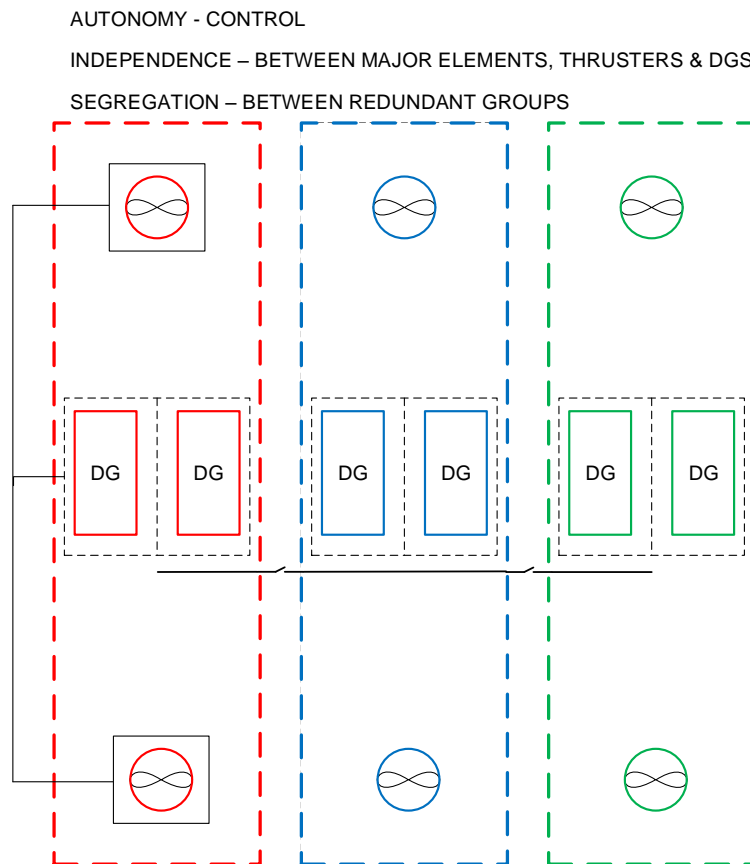
Figure 5-1 Redundancy Design Intent in DP Power Plant
