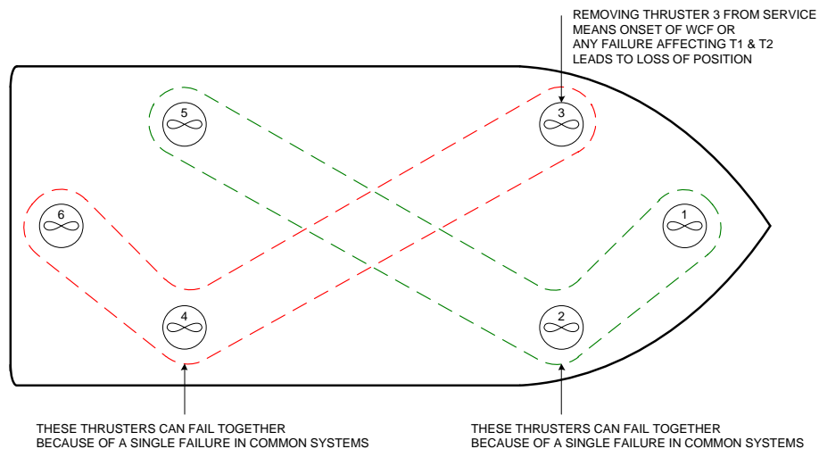
Figure 2-2 Thruster Arrangement
